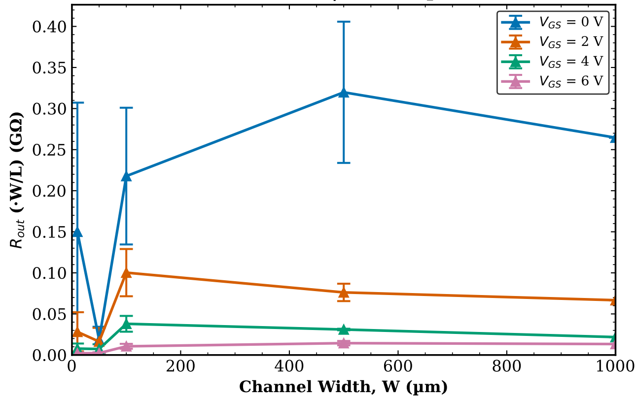
All Chips - Combined R_{out} vs W | L = 20\text{ }\mu\text{m}
